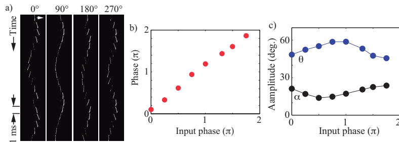
Fig. 2. Wing kinematics. a) High-speed video from four experiments at 100 Hz. Phase offset denoted above. Frames are 1 ms apart. b) Input and measured phase difference in wing stroke and pitch. c) Peak-to-peak amplitude of wing stroke and amplitude of angle of attack.
