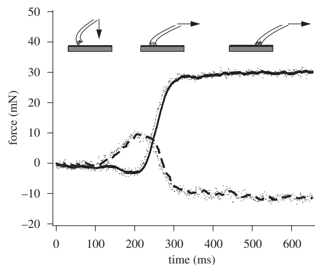
Figure 1. The tokay gecko (approx. 30 cm in length) possesses adhesive pads on the undersides of its toes (approx. 1 cm in length). Arrays of branched setae (approx. 110 \mu\text{m} in length) achieve intimate contact with surfaces to engage intermolecular van der Waals forces. Setae are adhesive only under the application of a shear force. Setae are first applied vertically to a surface and then sheared parallel to the surface. The setal shafts load elastically until the elastic component is saturated, at which point the setae slide across the substrate while remaining in adhesion. As the adhesive begins to slide (300 ms), friction and adhesion forces remain constant and do not exhibit any notable decrease, uncharacteristic of solid contact mechanics. The solid line represents friction and the dashed line adhesion. Note that for normal force, adhesion is negative while compression is positive.
